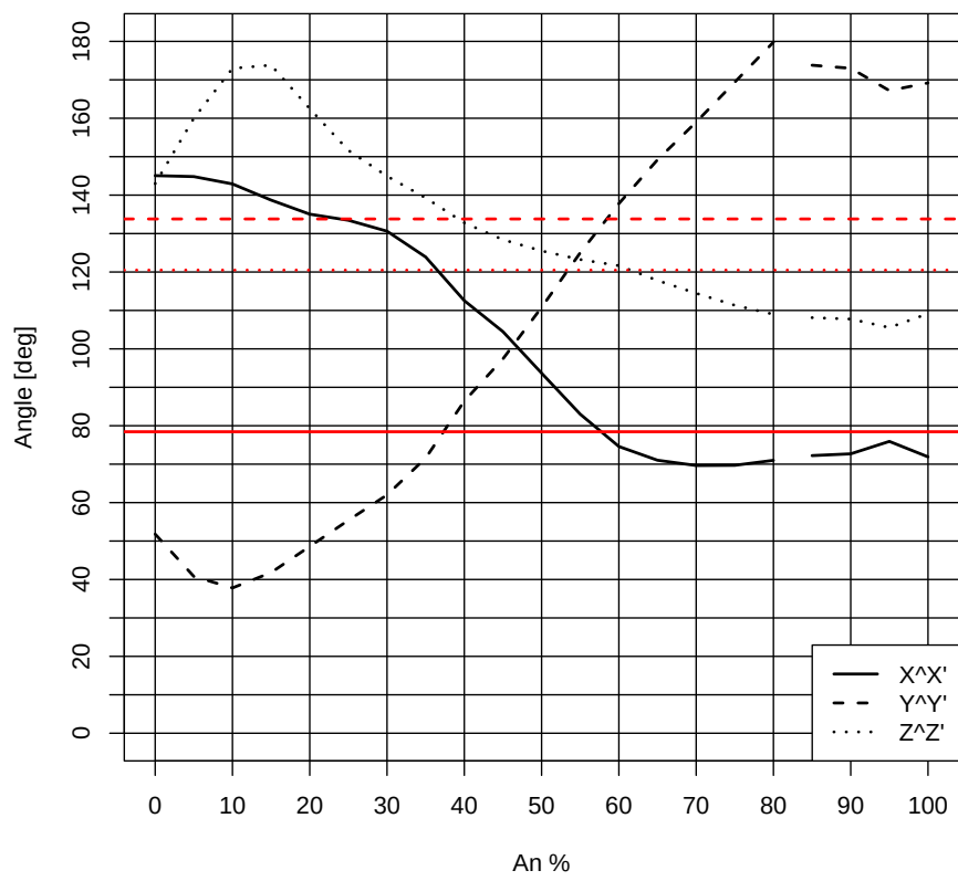
Figure 2: Angles between the principal axes according to the Karlsbad law.
