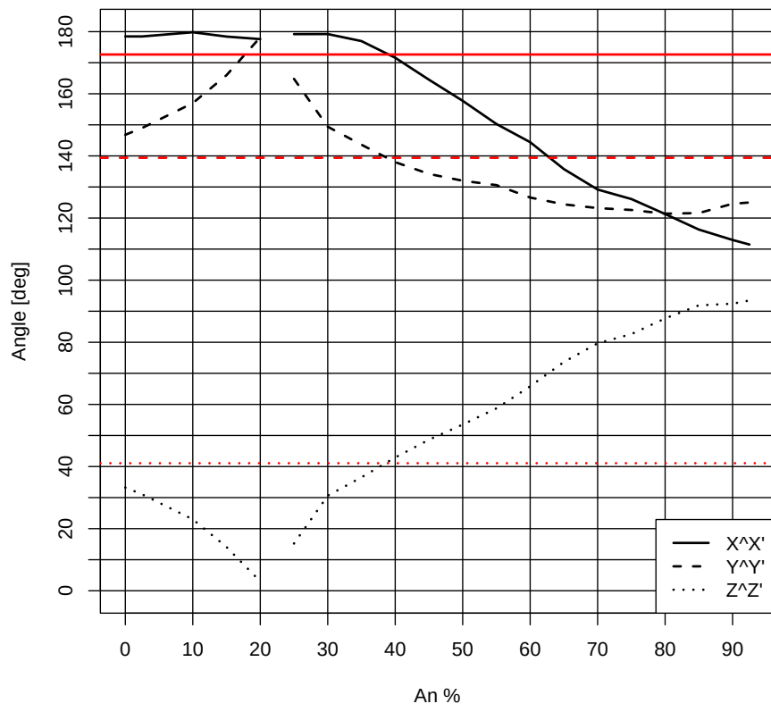
Figure 2: Angles between the principal axes according to the Albit law.
